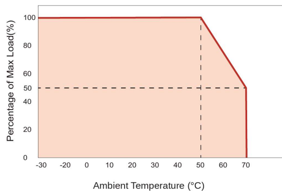
Derating Curve
